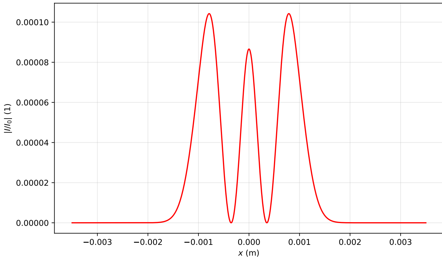
Intensity profile I(x, y = 0, z = 0.318)/I_0 , P_{in}=2.0P_{cr} , artificial time
